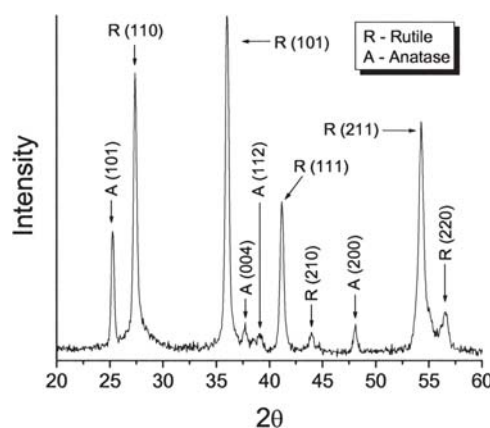
Fig. 4 XRD pattern of the HVOF sprayed nanostructured titania coating
