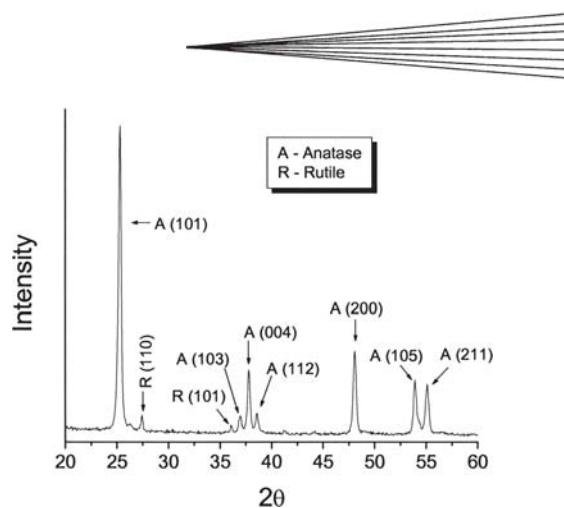
Fig. 3 XRD pattern of the nanostructured titania feedstock powder
