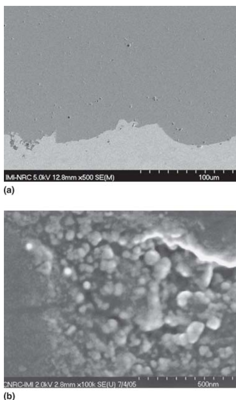
Fig. 2 (a) Cross section of the HVOF sprayed titania coating made from the nanostructured feedstock on the Ti-6Al-4V substrate. (b) Higher magnification view of (a) showing a nanostructured zone (formed by a nanostructured agglomerate that was semimolten in the spray jet)
