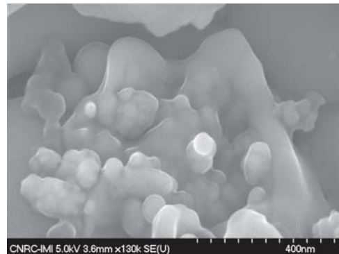
Fig. 5 A nanotextured region on the surface of the HVOF sprayed nanostructured titania coating
